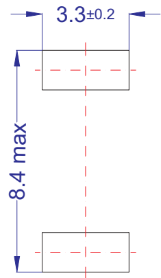
SMC DO-214 AB
