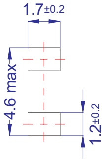
Mini-Melf DO-213 AA
