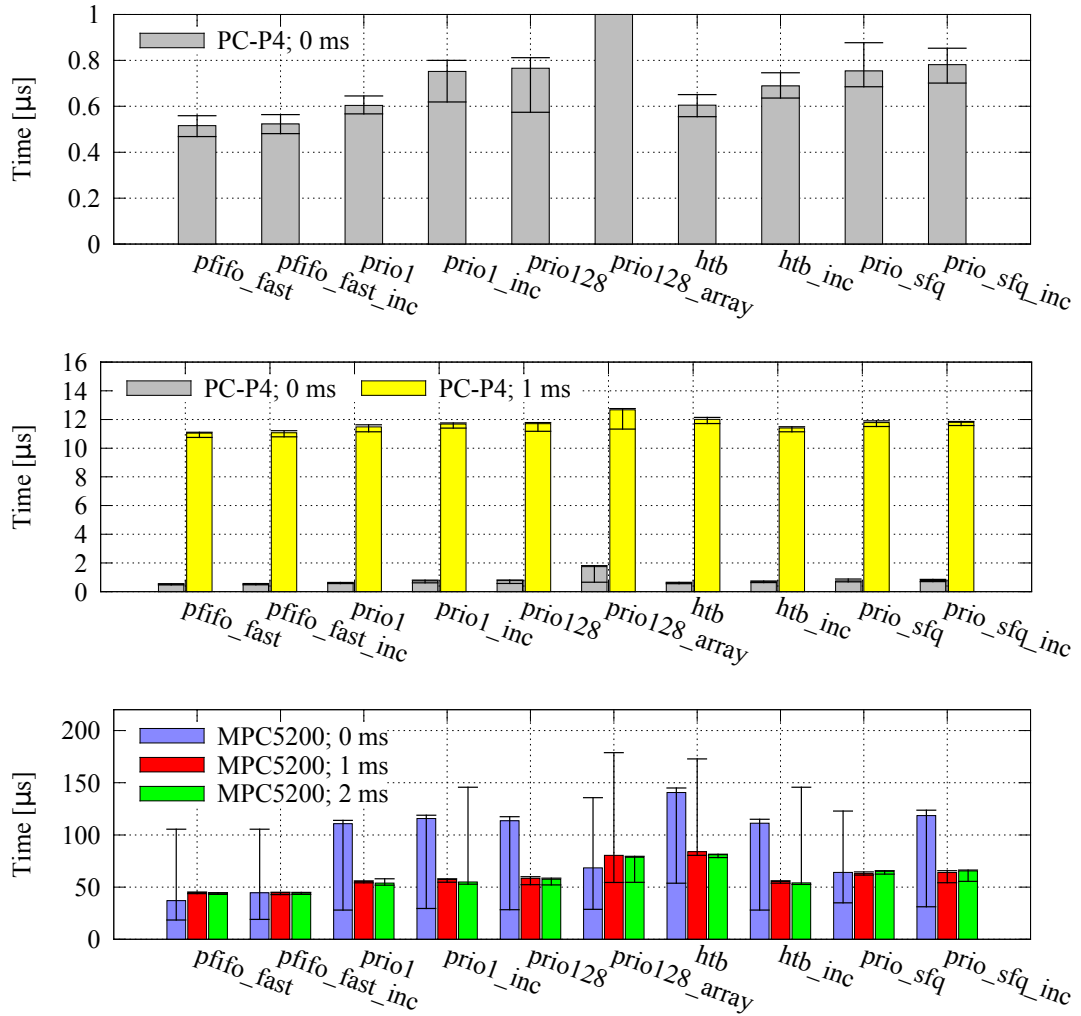
Figure 4.7.: Time spent in can_send() (minimum, 50 th and 90 th percentiles) with real CAN interface depending on qdisc configuration, platform and traffic. CAN filter was compiled with SFF rules stored in a bitmap except from prio128_array experiment where the filtering rules were stored in an array.
