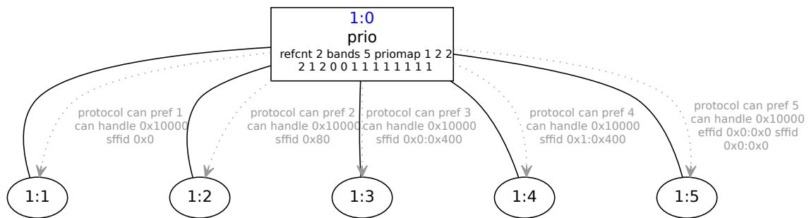
Figure A.1.: Prio qdisc with 5 classes.
