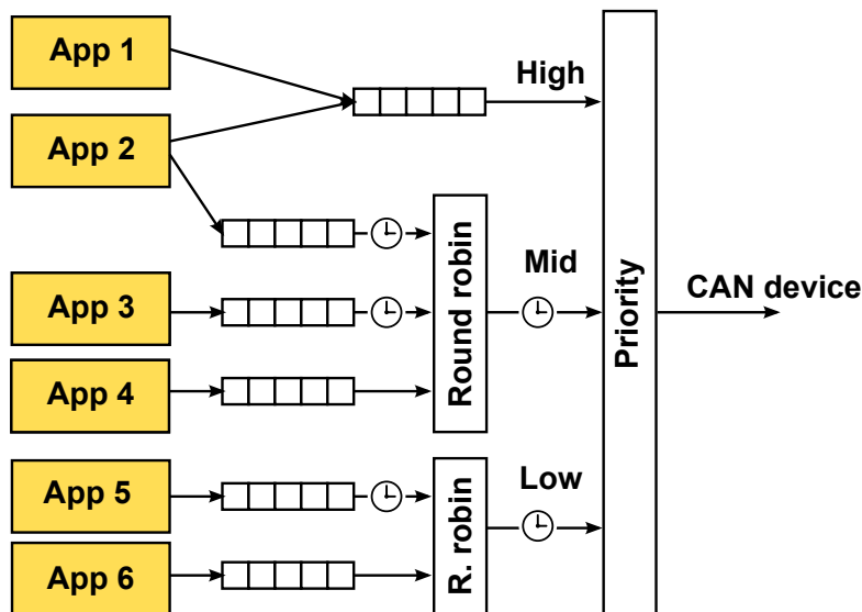
Figure 1.1.: Ideal CAN queueing discipline.
