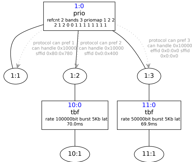
Figure A.2.: Prio qdisc with TBF child qdiscs.
