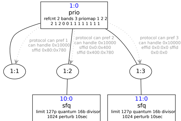
Figure A.3.: Prio qdisc with SFQ child-qdiscs.
