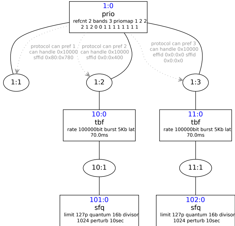
Figure A.4.: Prio qdisc with HTB child-qdiscs which have SFQ child-qdiscs.
