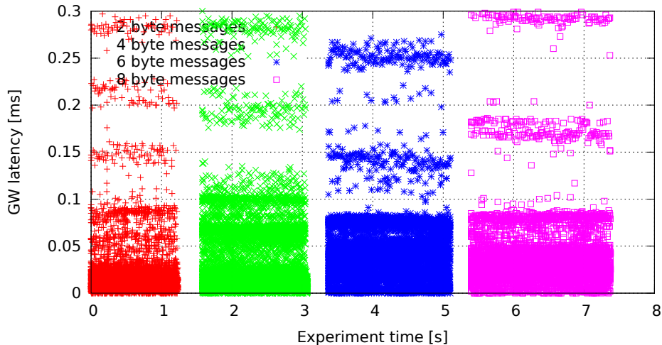
Single GW rule for all messages, no modifications (GW kernel rtems4.10-midam, Traffic flood, Load eth)
