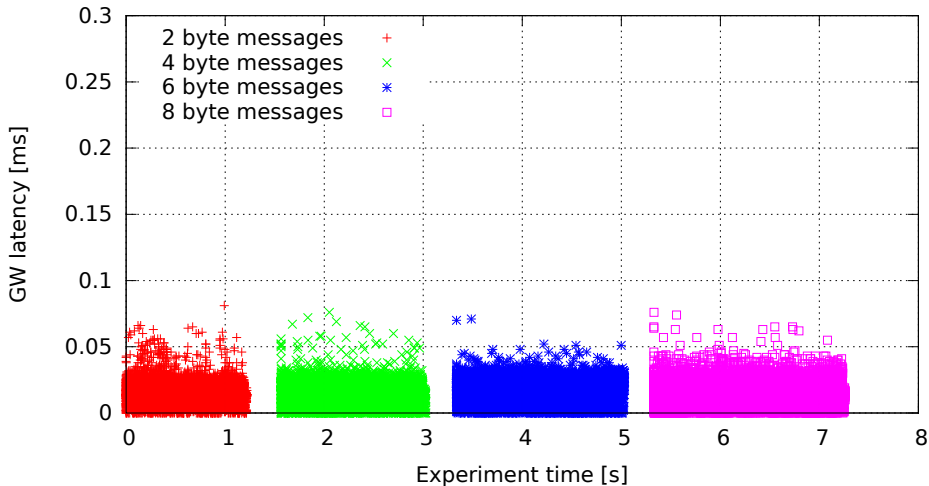
Single GW rule for all messages, no modifications, high (soft)irq task priority (GW kernel rtems4.10-midam, Traffic flood, Load eth)
