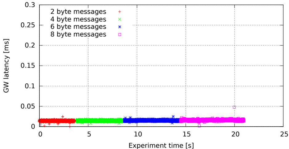
Single GW rule for all messages, no modifications, high (soft)irq task priority (GW kernel rtems4.10-midam, Traffic 50, Load none)
