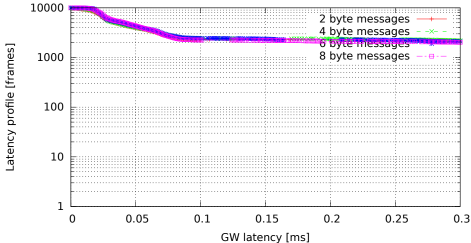
Single GW rule for all messages, no modifications (GW kernel rtems4.10-midam, Traffic 50, Load eth)
