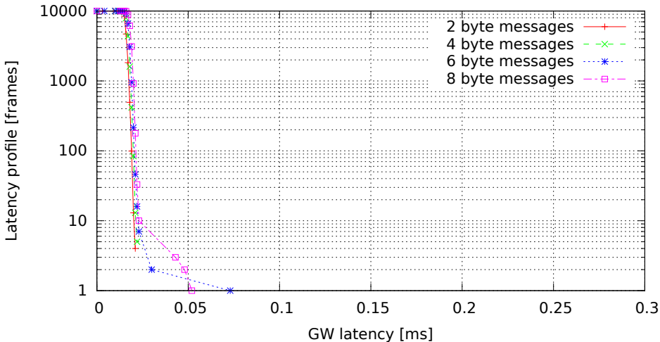
Single GW rule for all messages, no modifications, high (soft)irq task priority (GW kernel rtems4.10-midam, Traffic 50, Load cpu)
