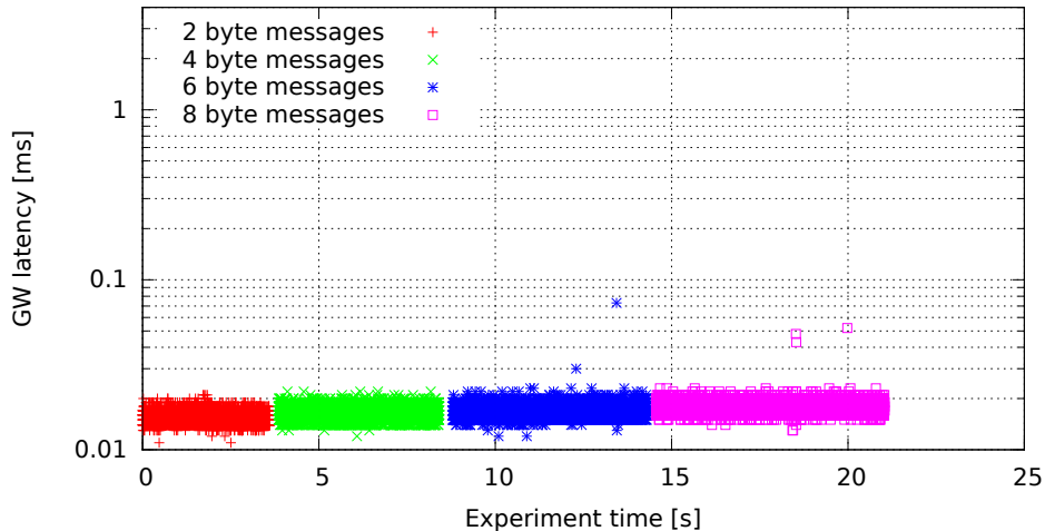
Single GW rule for all messages, no modifications, high (soft)irq task priority (GW kernel rtems4.10-midam, Traffic 50, Load cpu)
