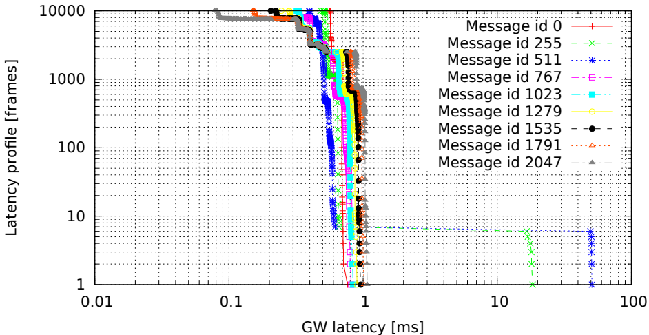
2048 GW rules (one per id, mask 0x7FF), no modifications (GW kernel 3.4.33-rt47-00004-gc58c9ae, Traffic oneatatime, Load none)
