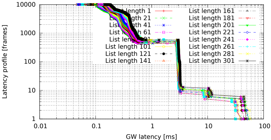
Different lengths of filter list, only the last one matches (GW kernel 3.4.33-rt47-00004-gc58c9ae, Traffic oneatatime, Load eth)
