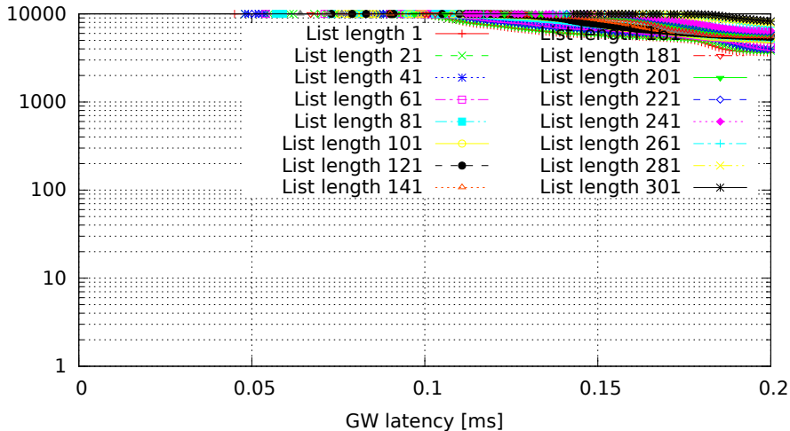
Different lengths of filter list, only the last one matches (GW kernel 3.4.33-rt47-00004-gc58c9ae, Traffic oneatime, Load eth)
