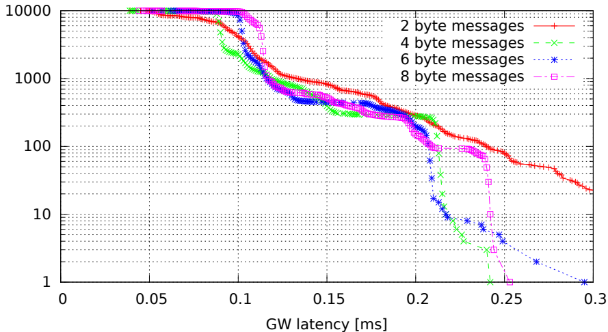
Single GW rule for all messages, no modifications (GW kernel 3.4.33-rt47-00004-gc58c9ae, Traffic flood, Load none)
