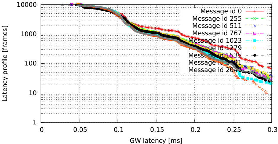
2048 GW rules (one per id, mask C00007FF), no modifications (GW kernel 3.4.33-rt47-00004-gc58c9ae, Traffic flood, Load none)
