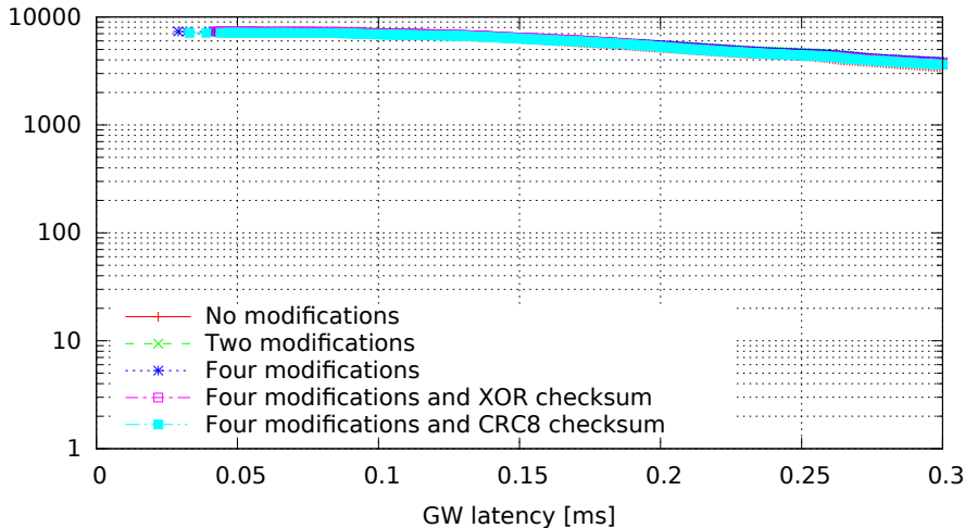
Single GW rule for all messages with modifications, 8 byte messages (GW kernel 3.4.33-rt47-00004-gc58c9ae, Traffic flood, Load eth)
