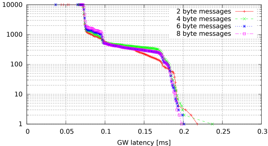
Single GW rule for all messages, no modifications (GW kernel 3.4.33-rt47-00004-gc58c9ae, Traffic 50, Load none)
