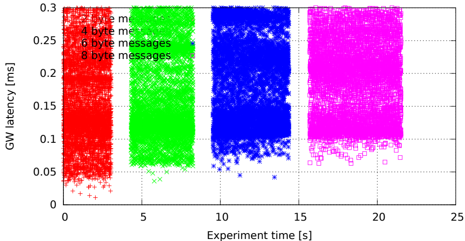
Single GW rule for all messages, no modifications (GW kernel 3.4.33-rt47-00004-gc58c9ae, Traffic 50, Load eth)
