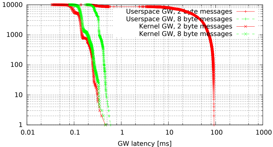
Kernel vs. userspace GW, no modifications (GW kernel 3.4.33-rt47-00004-gc58c9ae, Traffic 50, Load cpu)
