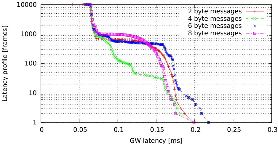
Single GW rule for all messages, no modifications, high (soft)irq task priority (GW kernel 3.0.7-rt20-00008-g0c18035, Traffic onetime, Load none)
