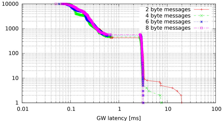
Single GW rule for all messages, no modifications (GW kernel 3.0.7-rt20-00008-g0c18035, Traffic onetotime, Load eth)
