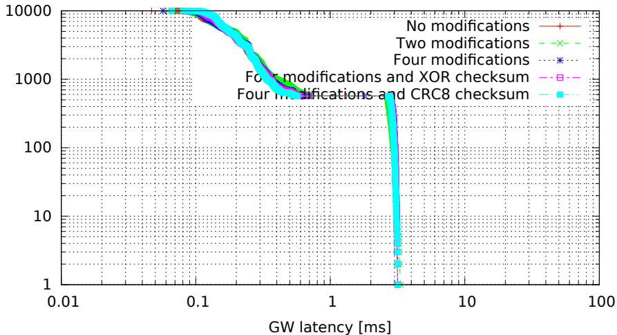
Single GW rule for all messages with modifications, 8 byte messages (GW kernel 3.0.7-rt20-00008-g0c18035, Traffic onetatime, Load eth)
