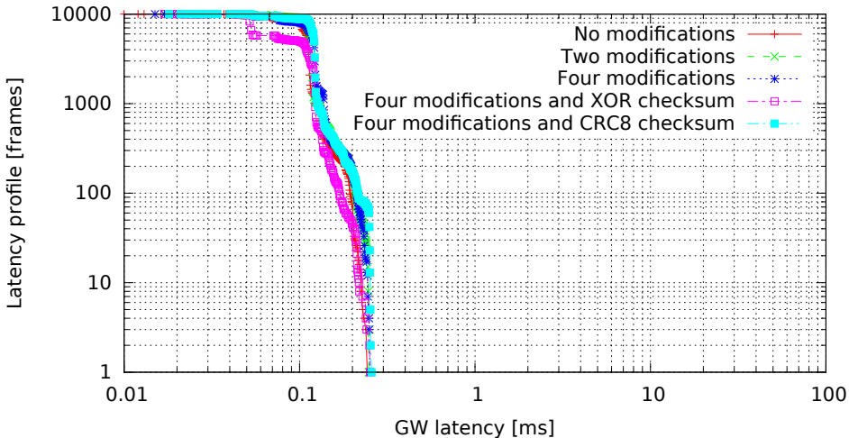
Single GW rule for all messages with modifications, 8 byte messages (GW kernel 3.0.7-rt20-00008-g0c18035, Traffic flood, Load none)
