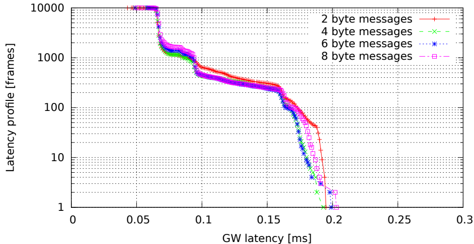
Single GW rule for all messages, no modifications (GW kernel 3.0.7-rt20-00008-g0c18035, Traffic 50, Load none)
