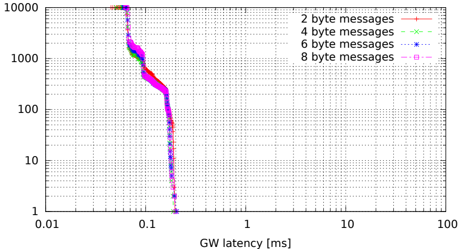
Single GW rule for all messages, no modifications, high (soft)irq task priority (GW kernel 3.0.7-rt20-00008-g0c18035, Traffic 50, Load none)
