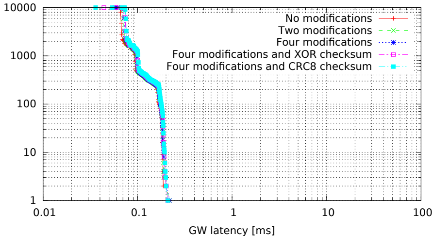
Single GW rule for all messages with modifications, 8 byte messages (GW kernel 3.0.7-rt20-00008-g0c18035, Traffic 50, Load none)
