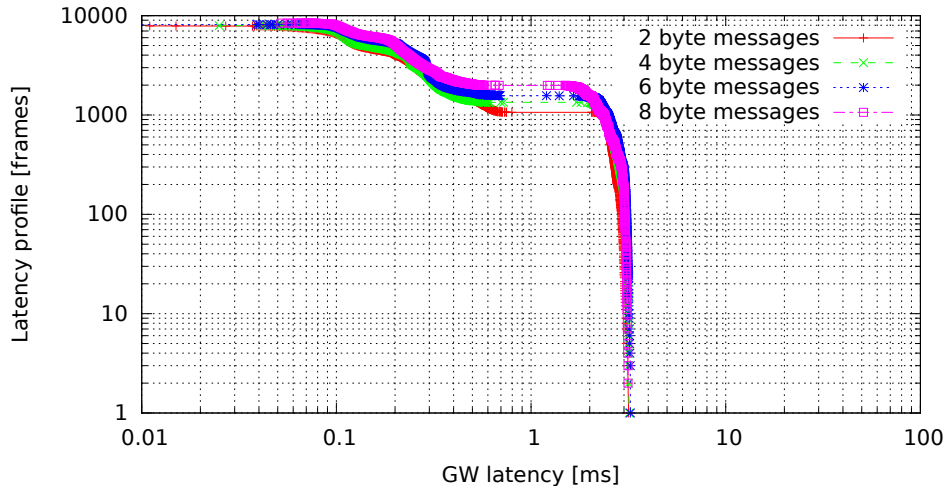
Single GW rule for all messages, no modifications (GW kernel 3.0.7-rt20-00008-g0c18035, Traffic 50, Load eth)
