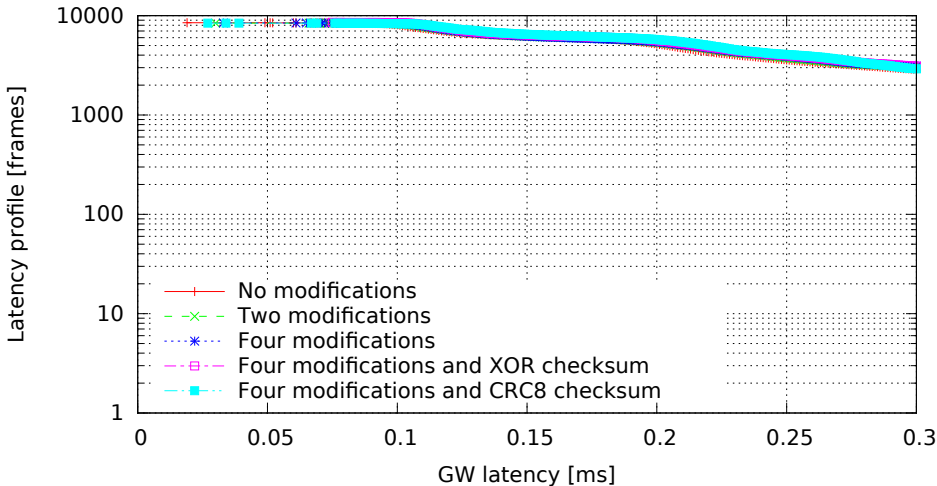
Single GW rule for all messages with modifications, 8 byte messages (GW kernel 3.0.7-rt20-00008-g0c18035, Traffic 50, Load eth)
