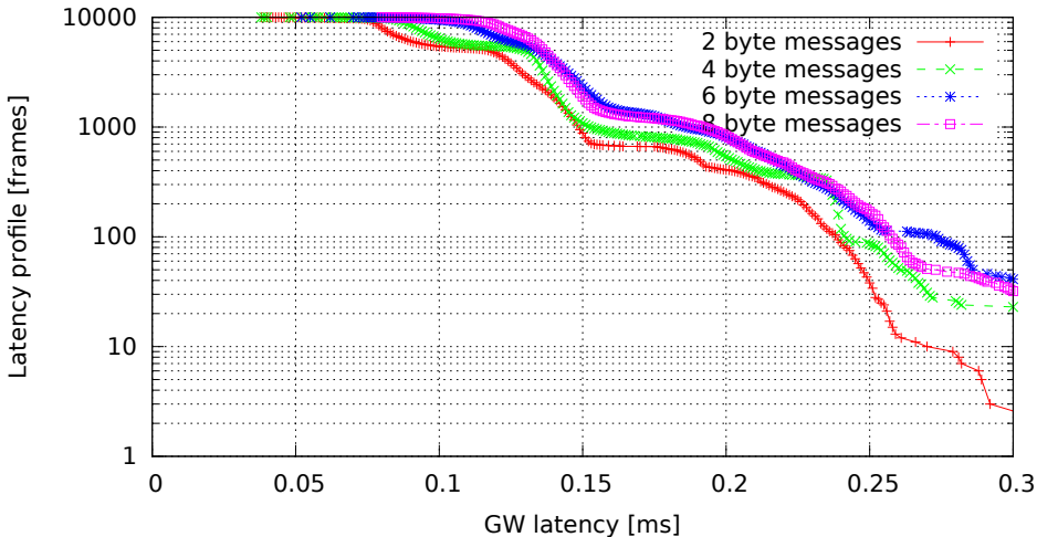
Single GW rule for all messages, no modifications, high (soft)irq task priority (GW kernel 3.0.7-rt20-00008-g0c18035, Traffic 50, Load cpu)
