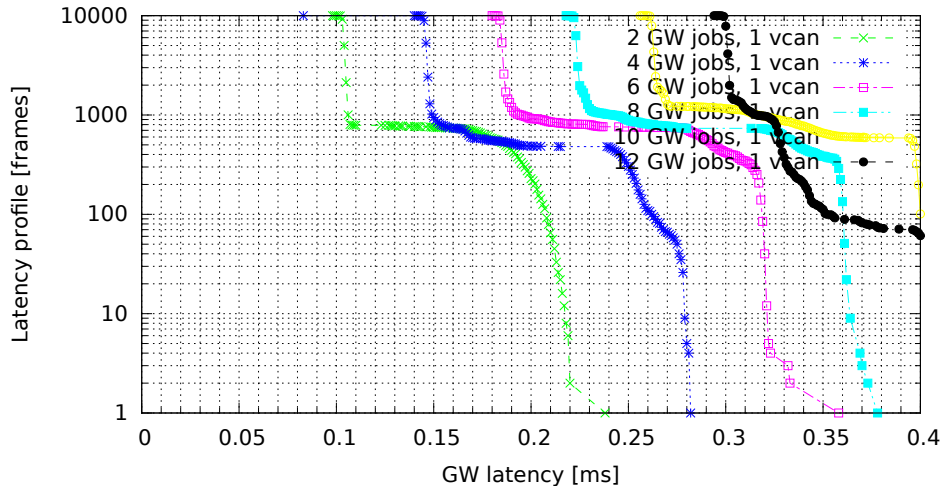
Chained GWs on a single VCAN interface (GW kernel 3.0.4-rt14-00008-gb2052fd, Traffic oneatatime, Load none)
