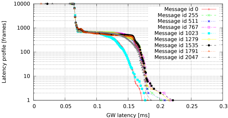
2048 GW rules (one per id, mask C00007FF), no modifications (GW kernel 3.0.4-rt14-00008-gb2052fd, Traffic oneatatime, Load none)
