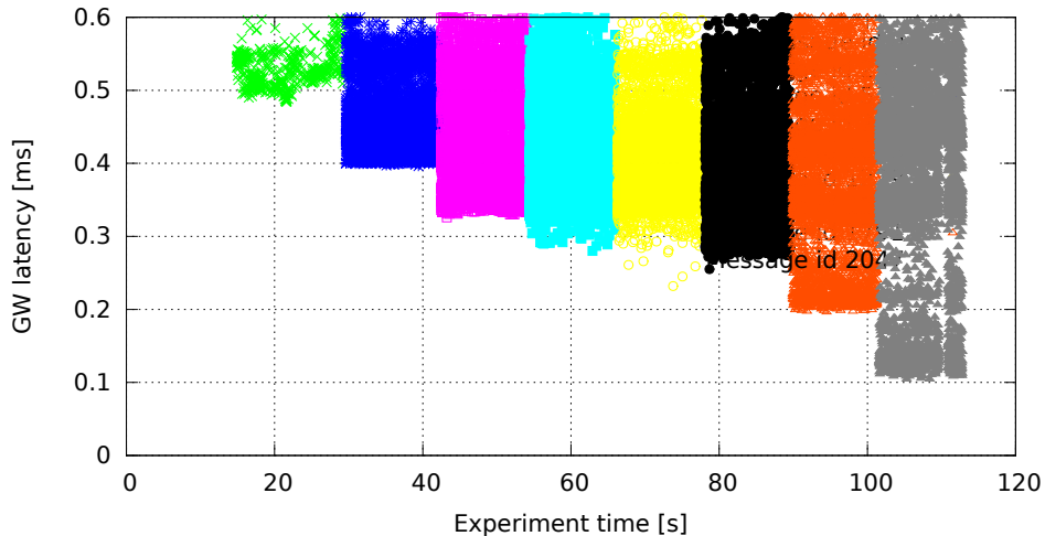
2048 GW rules (one per id, mask 0x7FF), no modifications (GW kernel 3.0.4-rt14-00008-gb2052fd, Traffic oneatatime, Load eth)
