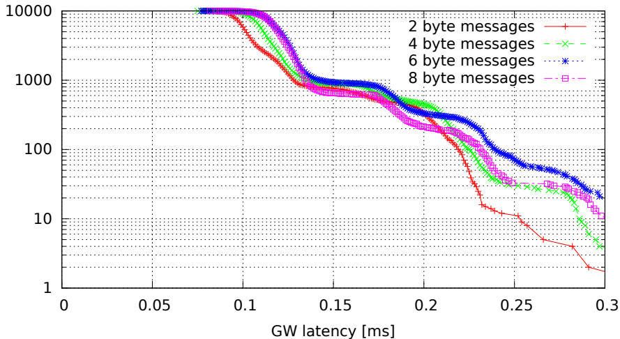
Single GW rule for all messages, no modifications (GW kernel 3.0.4-rt14-00008-gb2052fd, Traffic oneatatime, Load cpu)
