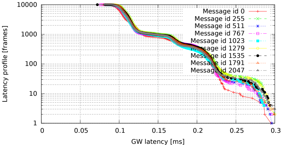
2048 GW rules (one per id, mask C00007FF), no modifications (GW kernel 3.0.4-rt14-00008-gb2052fd, Traffic oneatatime, Load cpu)
