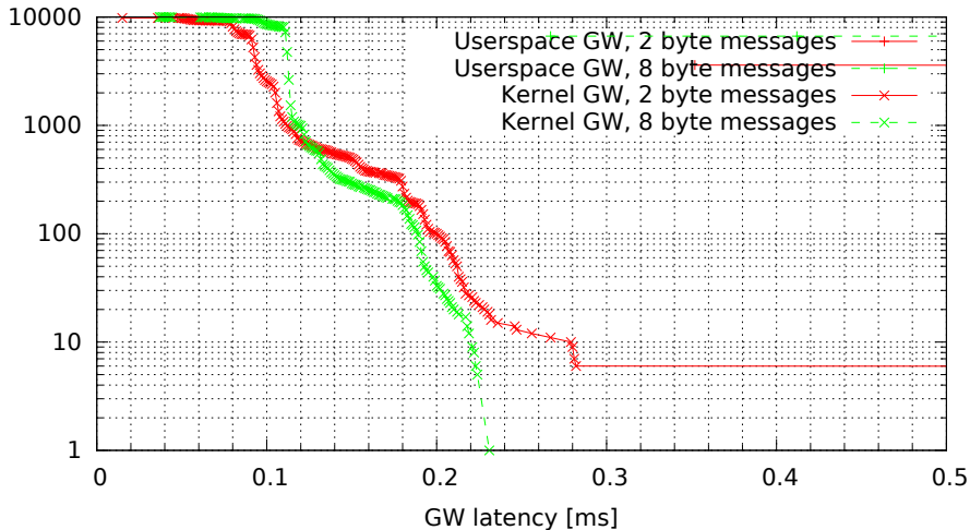
Kernel vs. userspace GW, no modifications (GW kernel 3.0.4-rt14-00008-gb2052fd, Traffic flood, Load none)
