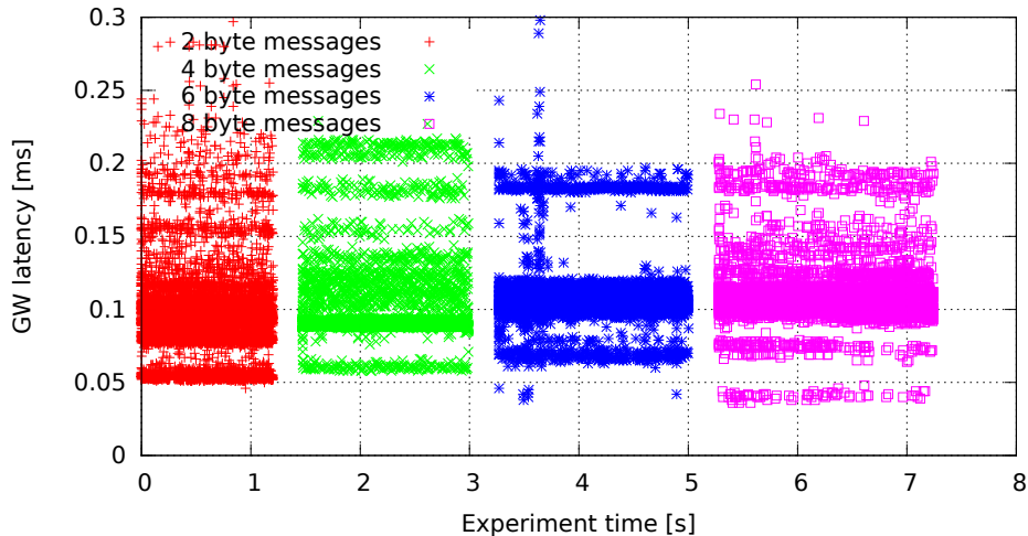
Single GW rule for all messages, no modifications (GW kernel 3.0.4-rt14-00008-gb2052fd, Traffic flood, Load none)
