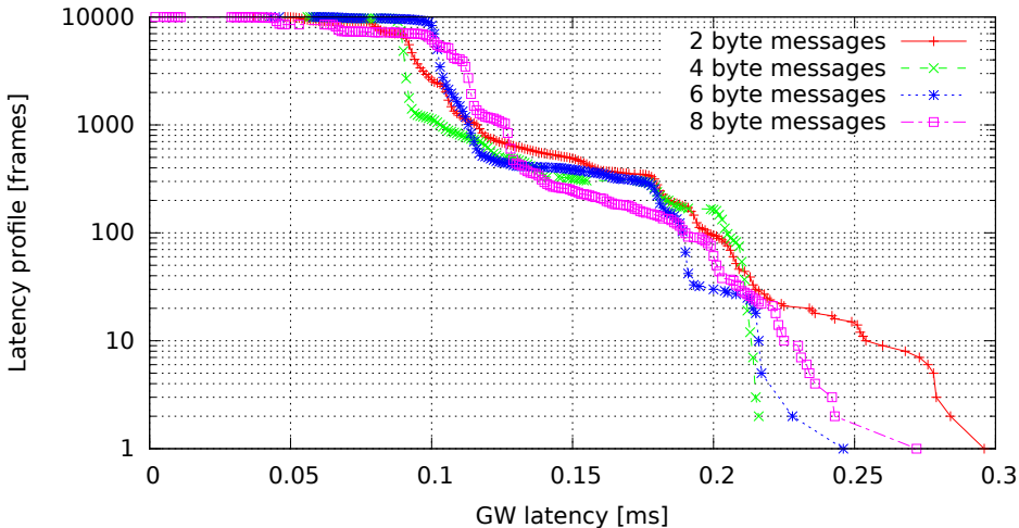
Single GW rule for all messages, no modifications, high (soft)irq task priority (GW kernel 3.0.4-rt14-00008-gb2052fd, Traffic flood, Load none)
