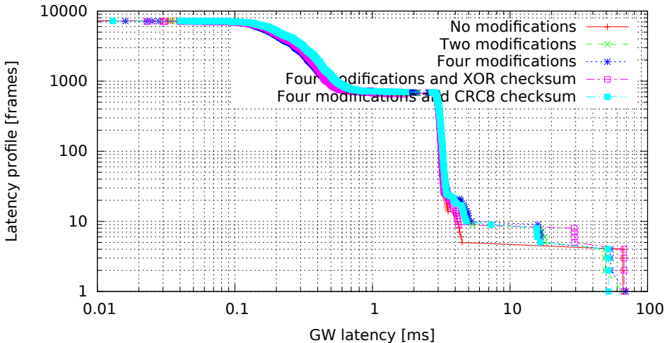
Single GW rule for all messages with modifications, 8 byte messages (GW kernel 3.0.4-rt14-00008-gb2052fd, Traffic flood, Load eth)
