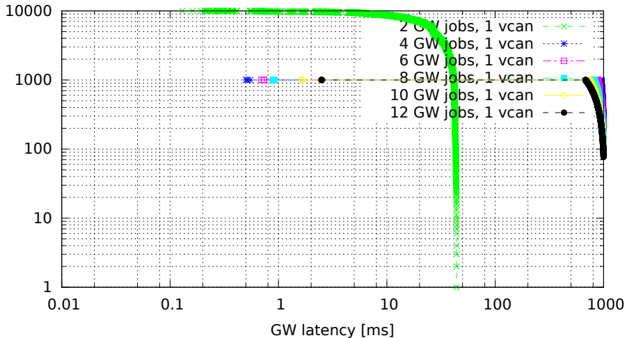
Chained GWs on a single VCAN interface (GW kernel 3.0.4-rt14-00008-gb2052fd, Traffic flood, Load cpu)
