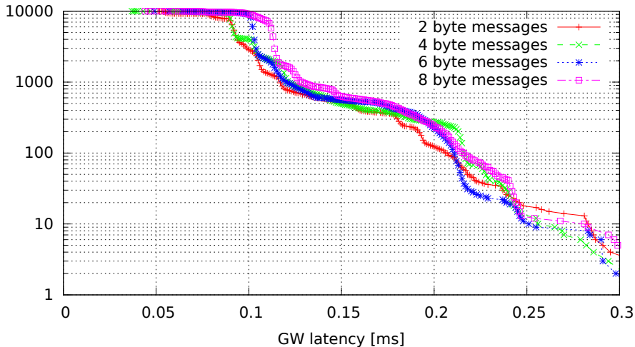
Single GW rule for all messages, no modifications, high (soft)irq task priority (GW kernel 3.0.4-rt14-00008-gb2052fd, Traffic flood, Load cpu)
