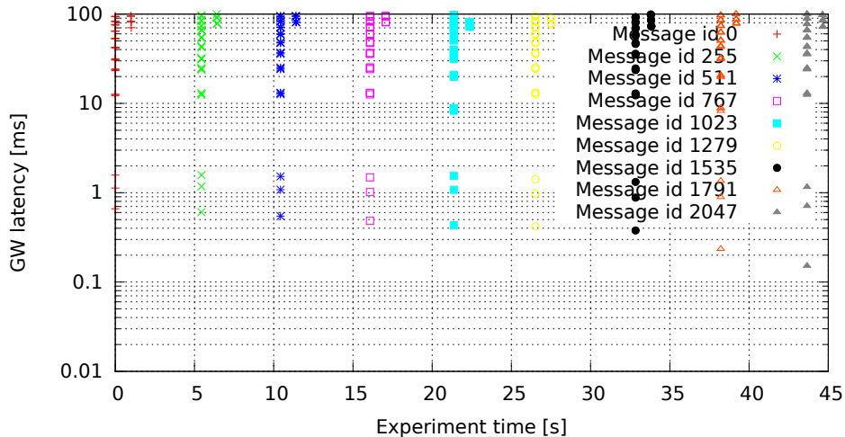
2048 GW rules (one per id, mask 0x7FF), no modifications (GW kernel 3.0.4-rt14-00008-gb2052fd, Traffic flood, Load cpu)
