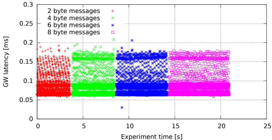
Single GW rule for all messages, no modifications (GW kernel 3.0.4-rt14-00008-gb2052fd, Traffic 50, Load none)
