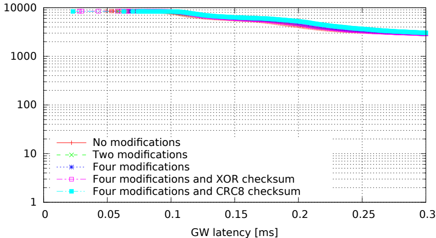
Single GW rule for all messages with modifications, 8 byte messages (GW kernel 3.0.4-rt14-00008-gb2052fd, Traffic 50, Load eth)
