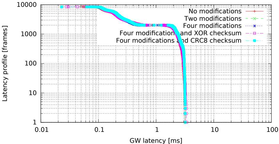
Single GW rule for all messages with modifications, 8 byte messages (GW kernel 3.0.4-rt14-00008-gb2052fd, Traffic 50, Load eth)
