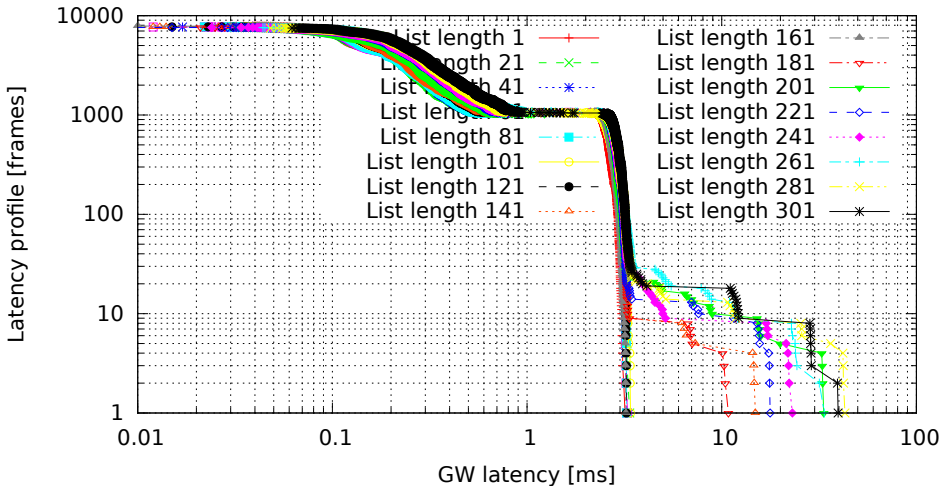
Different lengths of filter list, only the last one matches (GW kernel 3.0.4-rt14-00008-gb2052fd, Traffic 50, Load eth)
