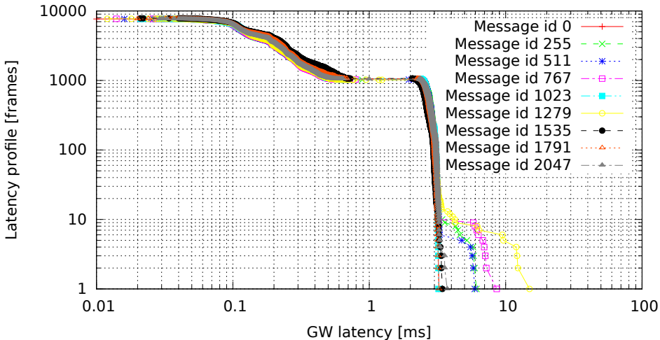
2048 GW rules (one per id, mask C00007FF), no modifications (GW kernel 3.0.4-rt14-00008-gb2052fd, Traffic 50, Load eth)
