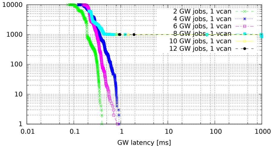
Chained GWs on a single VCAN interface (GW kernel 3.0.4-rt14-00008-gb2052fd, Traffic 50, Load cpu)
