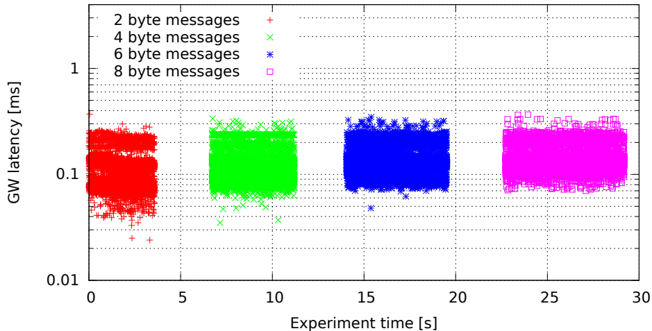
Single GW rule for all messages, no modifications (GW kernel 3.0.4-rt14-00008-gb2052fd, Traffic 50, Load cpu)
