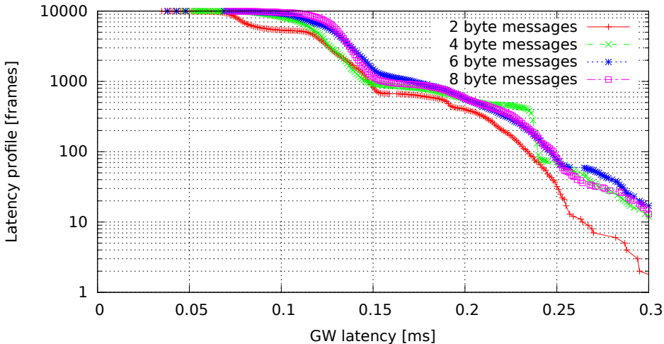
Single GW rule for all messages, no modifications, high (soft)irq task priority (GW kernel 3.0.4-rt14-00008-gb2052fd, Traffic 50, Load cpu)
