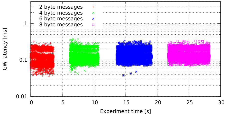
Single GW rule for all messages, no modifications, high (soft)irq task priority (GW kernel 3.0.4-rt14-00008-gb2052fd, Traffic 50, Load cpu)
