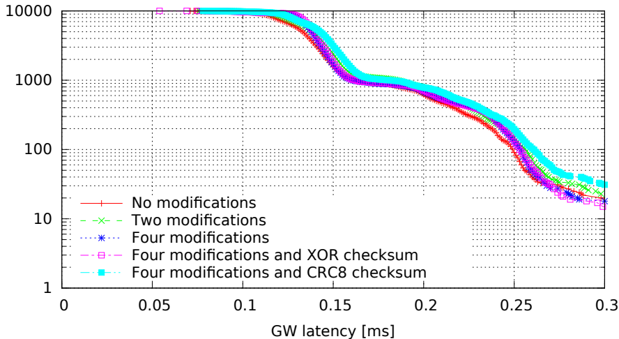
Single GW rule for all messages with modifications, 8 byte messages (GW kernel 3.0.4-rt14-00008-gb2052fd, Traffic 50, Load cpu)
