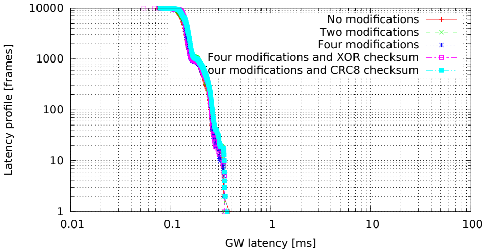
Single GW rule for all messages with modifications, 8 byte messages (GW kernel 3.0.4-rt14-00008-gb2052fd, Traffic 50, Load cpu)
